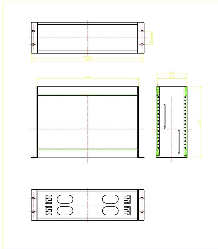
MPO Fiber Plugs For 3U 144 Core Frame
