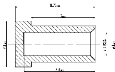
Figure-8: Cap
