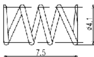
Figure-9: Spring
