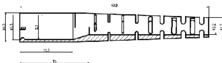
Figure-7: Boot
