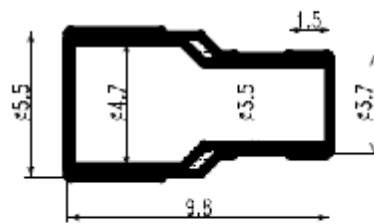
Figure-6:Crimp Ring
